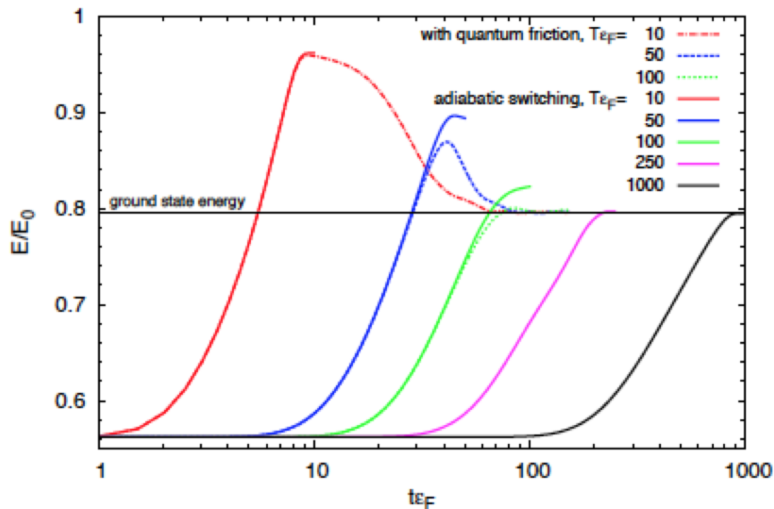
FIG. 3. (Color online) Ground state preparation of a trapped three-dimensional UFG gas from a translationally invariant (effectively two-dimensional) solution. The ground state can be prepared purely using adiabatic switching (solid lines) but the switching period can be dramatically reduced with local quantum friction. E_0 = \frac{3}{5}N\varepsilon_F , where N is number of particles and \varepsilon_F is Fermi energy in the center of initial solution. (See also the movie in [24].)
