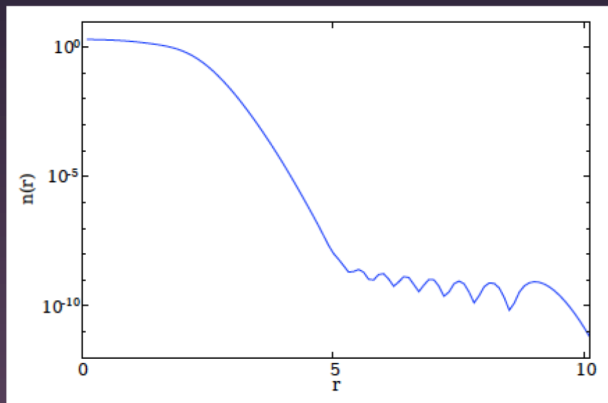
Our code with HO Basis
