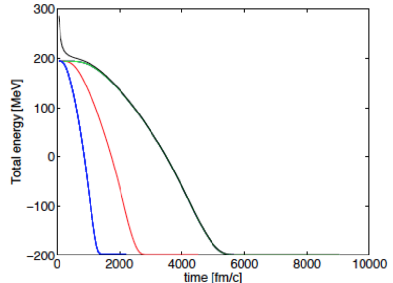
FIG. 2. (Color online) The total instantaneous energy of a system of twenty non-interacting neutrons evolving from an initial 3D harmonic oscillator potential to a final symmetrized Woods-Saxon potential. The curves correspond to quasi-adiabatic evolution with friction (1 - s_t)H_0 + s_t H_1 + U_t for various switching periods T (two-thirds of the simulation time) and just friction H_1 + U_t for the remaining third of the simulation. That the energy is constant during this time demonstrates that the ground state has been reached. Note: there are three curves for the longest T corresponding to different simulations with \{24^3, 32^3, 40^3\} lattices of 1 fm spacing: this demonstrates the infrared (IR) convergence.
