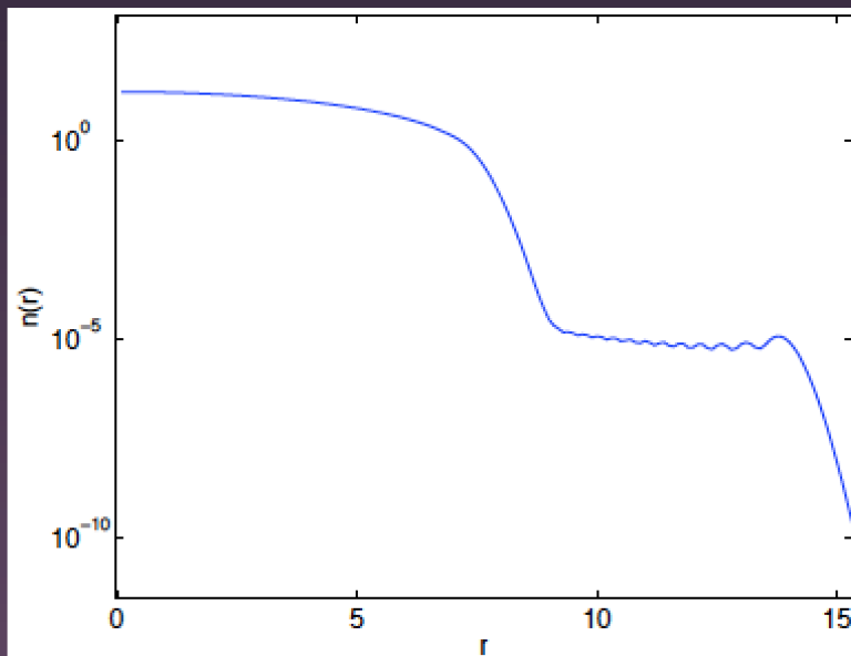
Grasso and Urban, BCS Code
