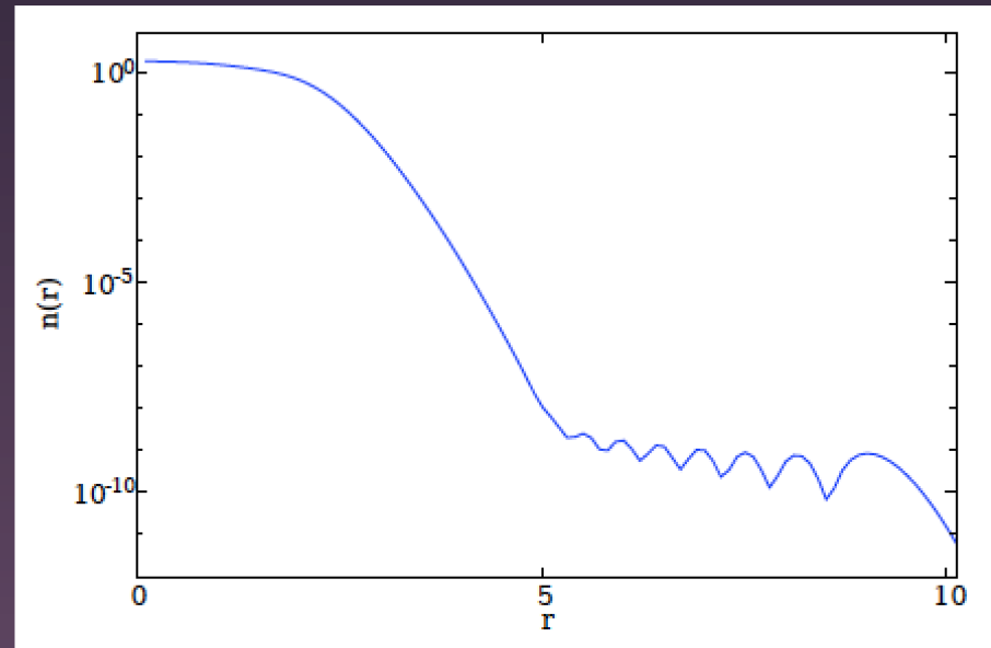
Our Unitary HO Basis Code
