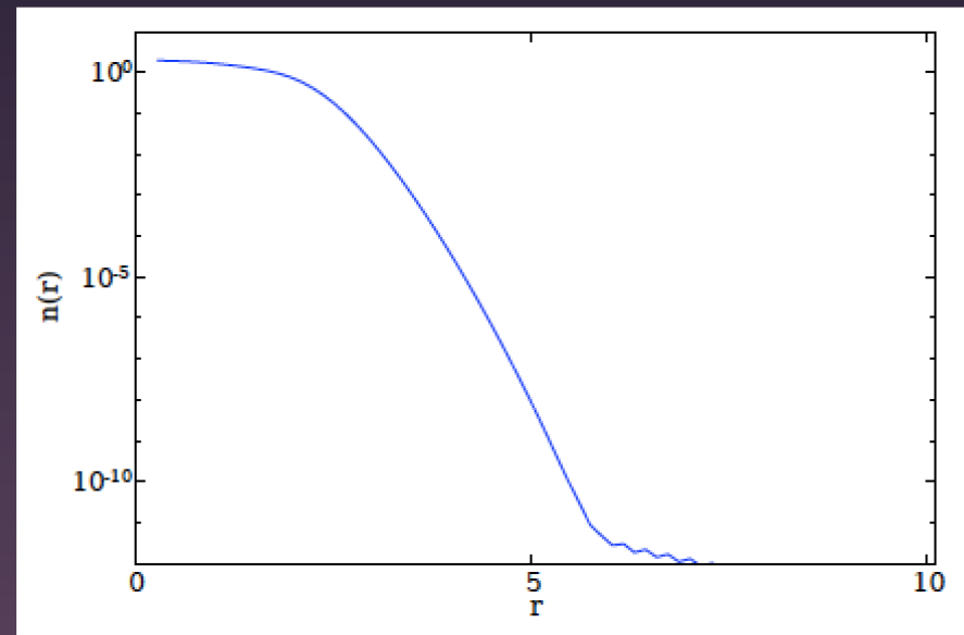
Our code with DVR Basis
