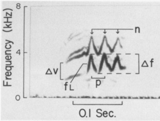
Fig. 1. Signature call of a Cliff Swallow chick showing the parameters evaluated. F -ratios (see text) are given after each parameter description. \Delta v = frequency difference between upper and lower voices ( F = 41.5 ). f_L = average frequency of the lower voice (74.0). p = period of frequency modulation (226). \Delta f = frequency difference between first modulation peak and valley of the lower voice (22.4). n = number of modulation cycles (51.7).
