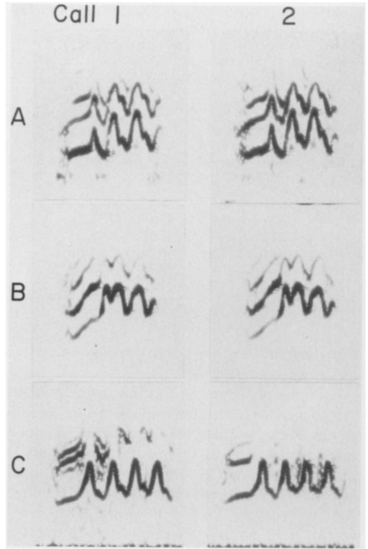
Fig. 2. Two signature calls each from three unrelated Cliff Swallow chicks (A, B, and C). Note the intraindividual consistency.
