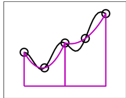
Composite Simpson's rule
