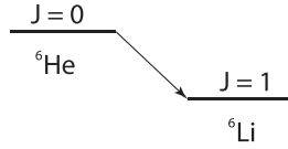
Fig. 3. Decay scheme for {}^6\text{He} .
