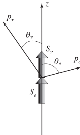
Fig. 2. Correlation between the initial polarization and the electron direction. In the decay of ^{60}\text{Co} , one unit of angular momentum is lost by the nucleus and has to be carried out by the leptons. Since the latter are spin-1/2 objects, they have to both align their spins in the direction of the initial polarization. This, in conjunction with the helicities of the particles, determines the emission probabilities.
